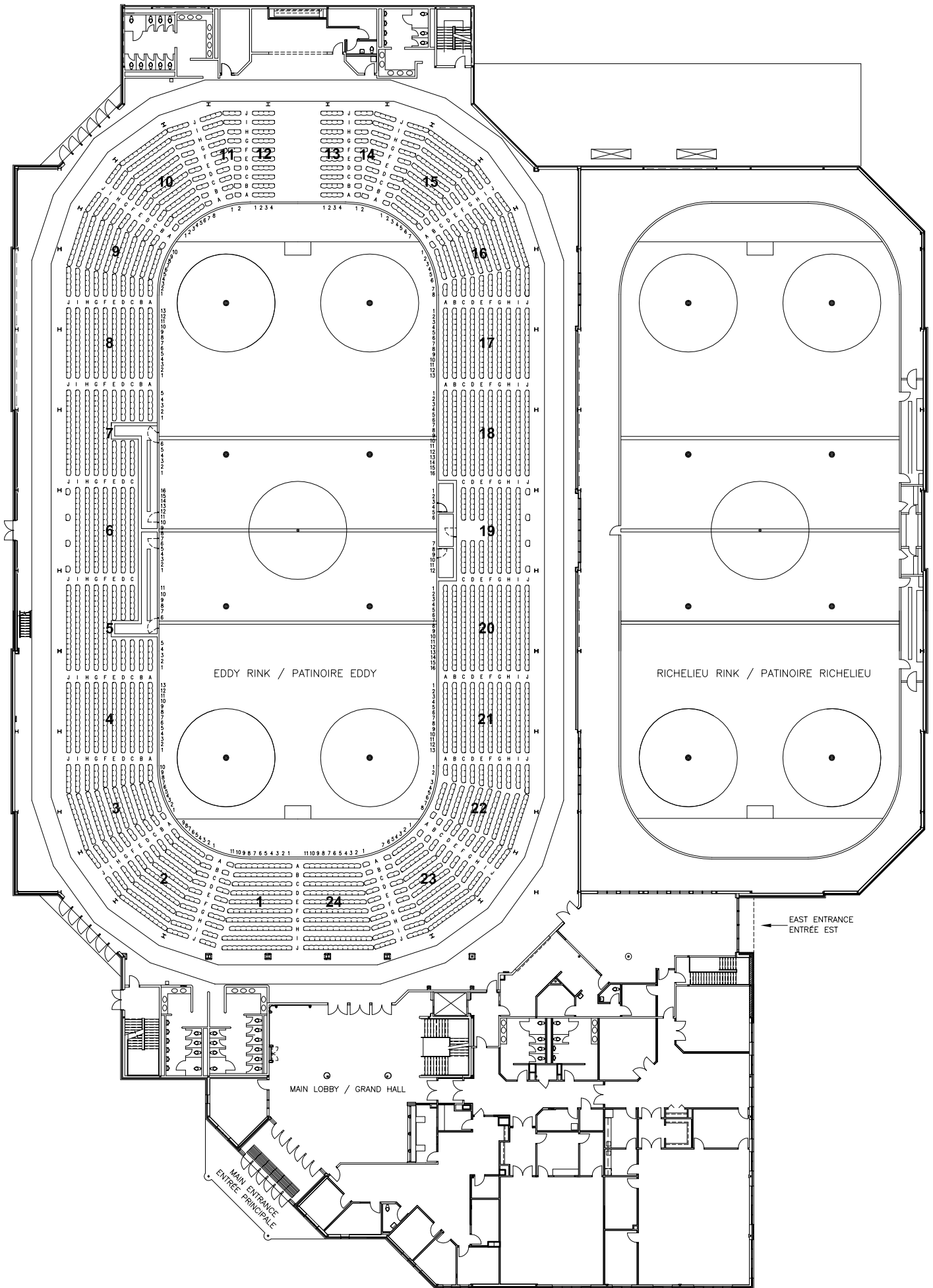
CONCOURSE LEVEL - SEATING LAYOUT NIVEAU DU GRAND HALL - PLAN DE LOCATION
